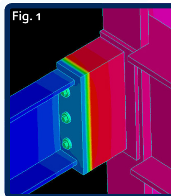
Fig. 1 shows the predicted temperature distribution with a Farrat TBL Structural Thermal Break and Thermal Isolating Washers. The temperature on the steelwork on the warm side of the cladding system is increased to 16.5°C and the heat loss (X-value) is reduced to 0.35 W/K, a 73% decrease in the heat loss.
